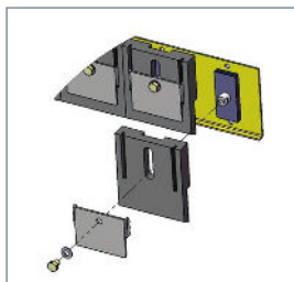
Individually adjustable rubber segments
